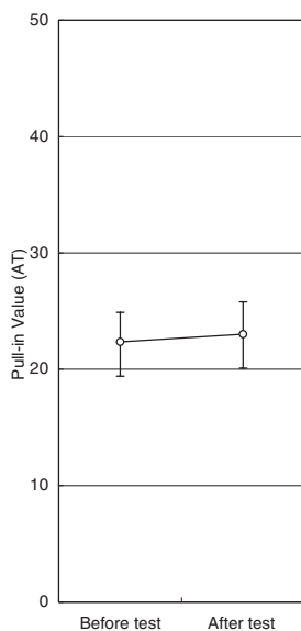
(1) Temperature cycle
